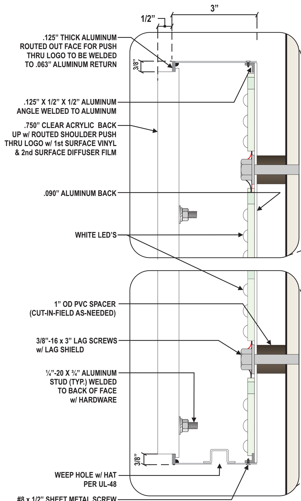
1 2 BLOW UP SECTION DETAIL Scale: 6"=1'-0"
