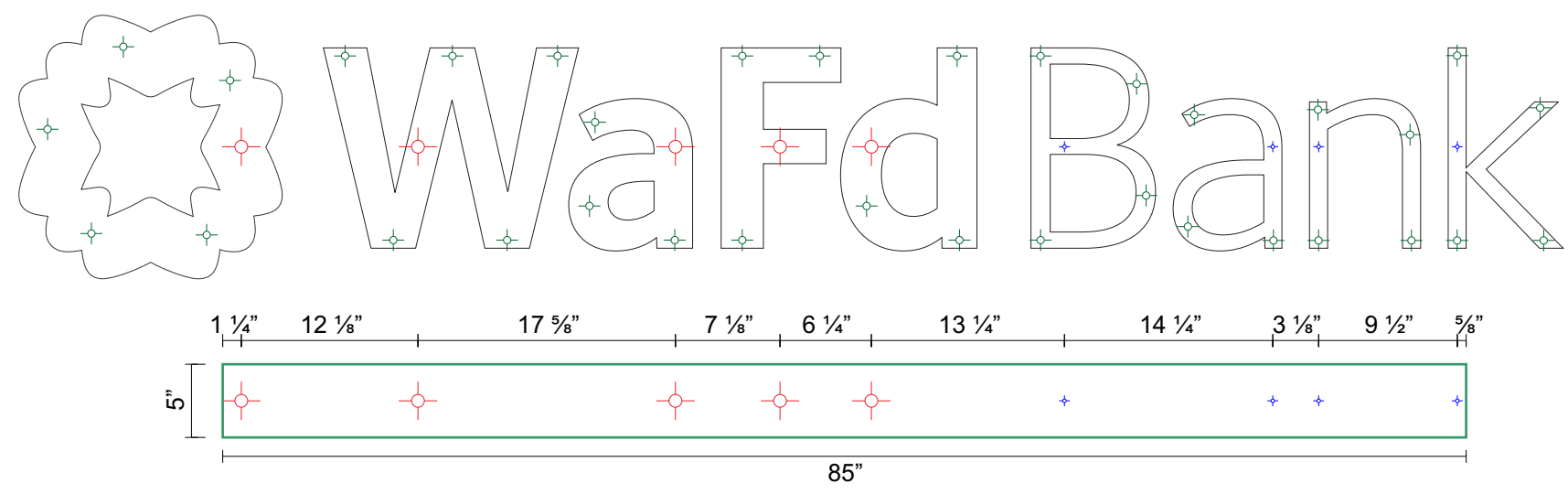
2 3 FRONT VIEW @ INSTALL PATTERN Scale: 1" = 1'-0"
