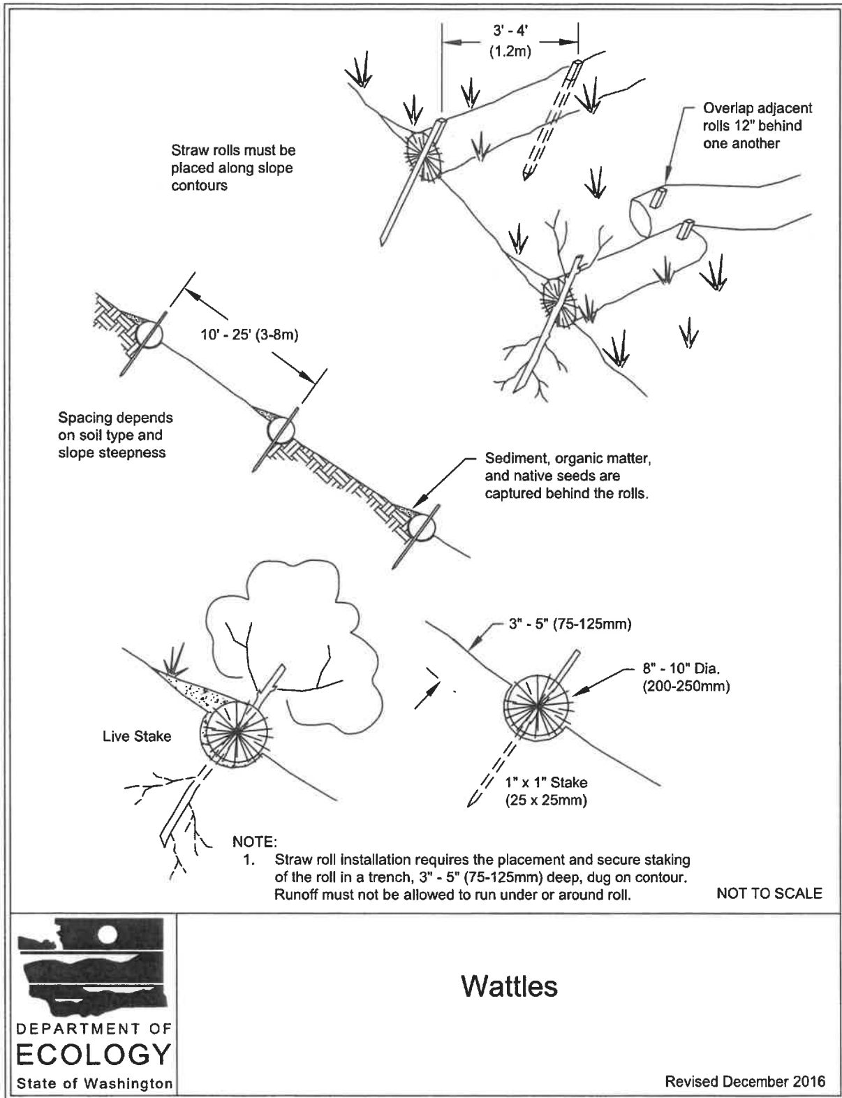
Figure II-4.24: Wattles
