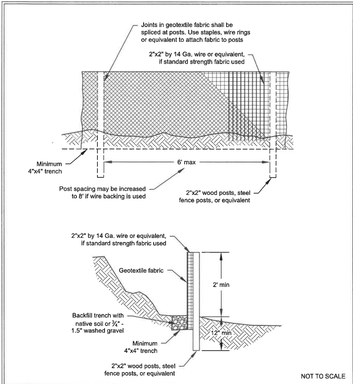
Figure II-4.22: Silt Fence
