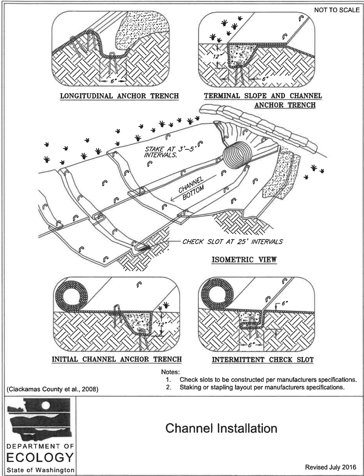
Figure II-4.3: Channel Installation
