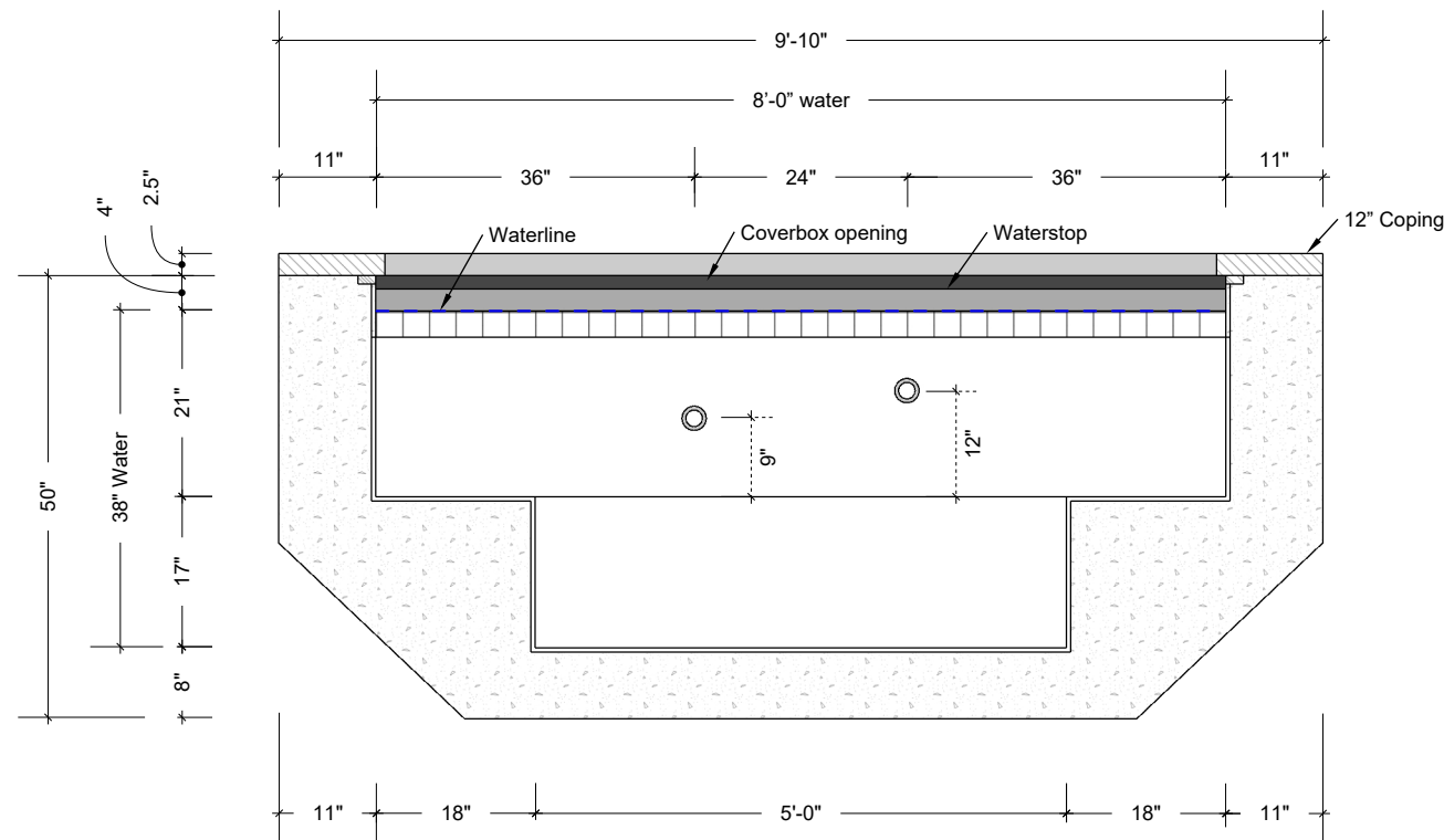
2 Spa Elevation PL6 Scale: 1/2" = 1FT Follow Measures
